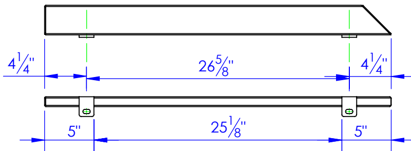
SUB-SIDERAIL 3349 LH SIDE RAIL 3350 LEFT HAND
